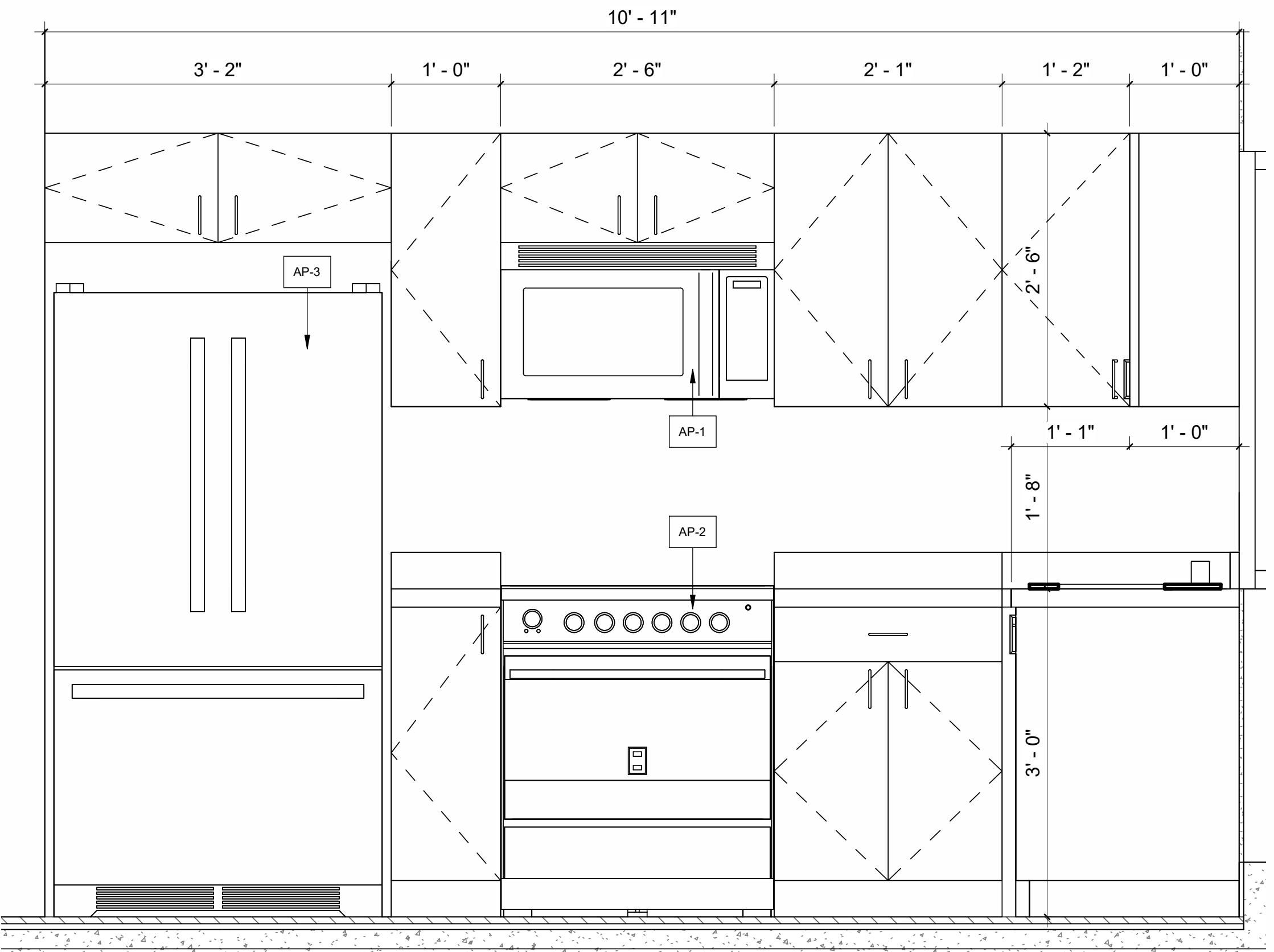
3 MILLWORK VIEW 1 1" = 1'-0"
