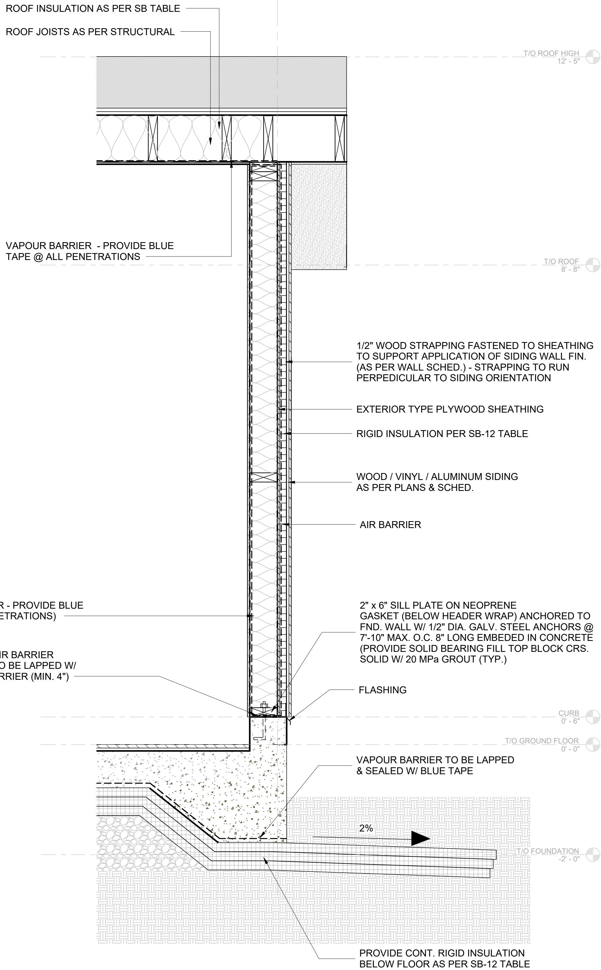
2 WALL SECTION 2 A-403 1" = 1'-0"
