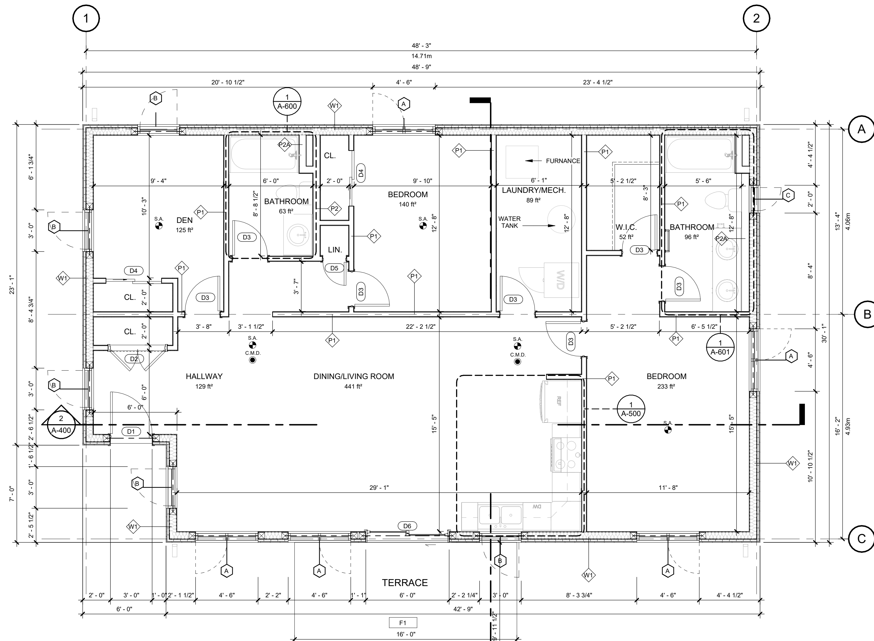
1 GROUND FLOOR A-100 1/4" = 1'-0"
