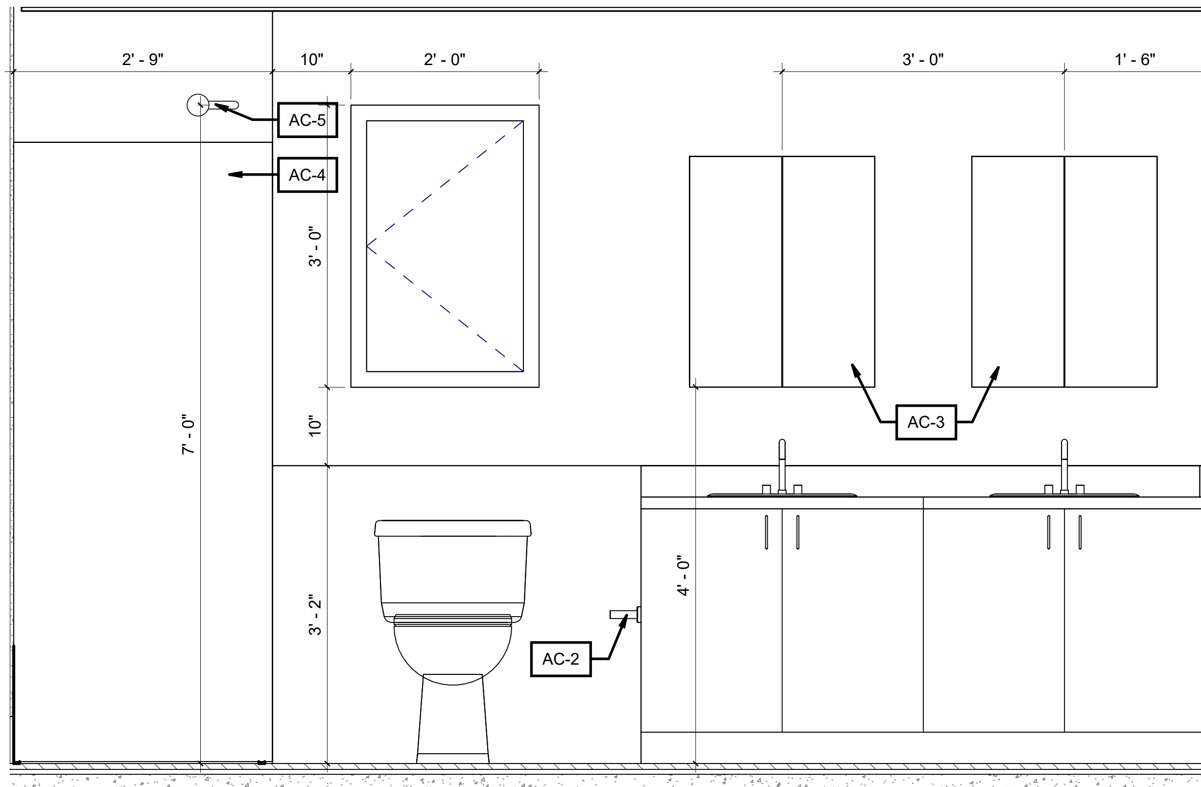
4 Elevation 2 - c A-601 1" = 1'-0"
