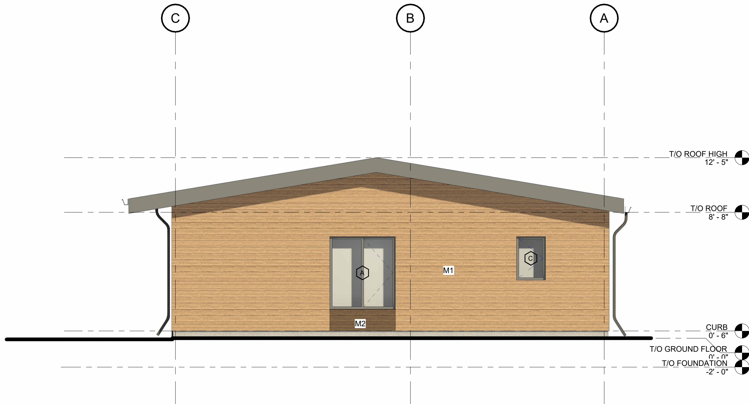
1 EAST ELEVATION A-300 1/4" = 1'-0"
