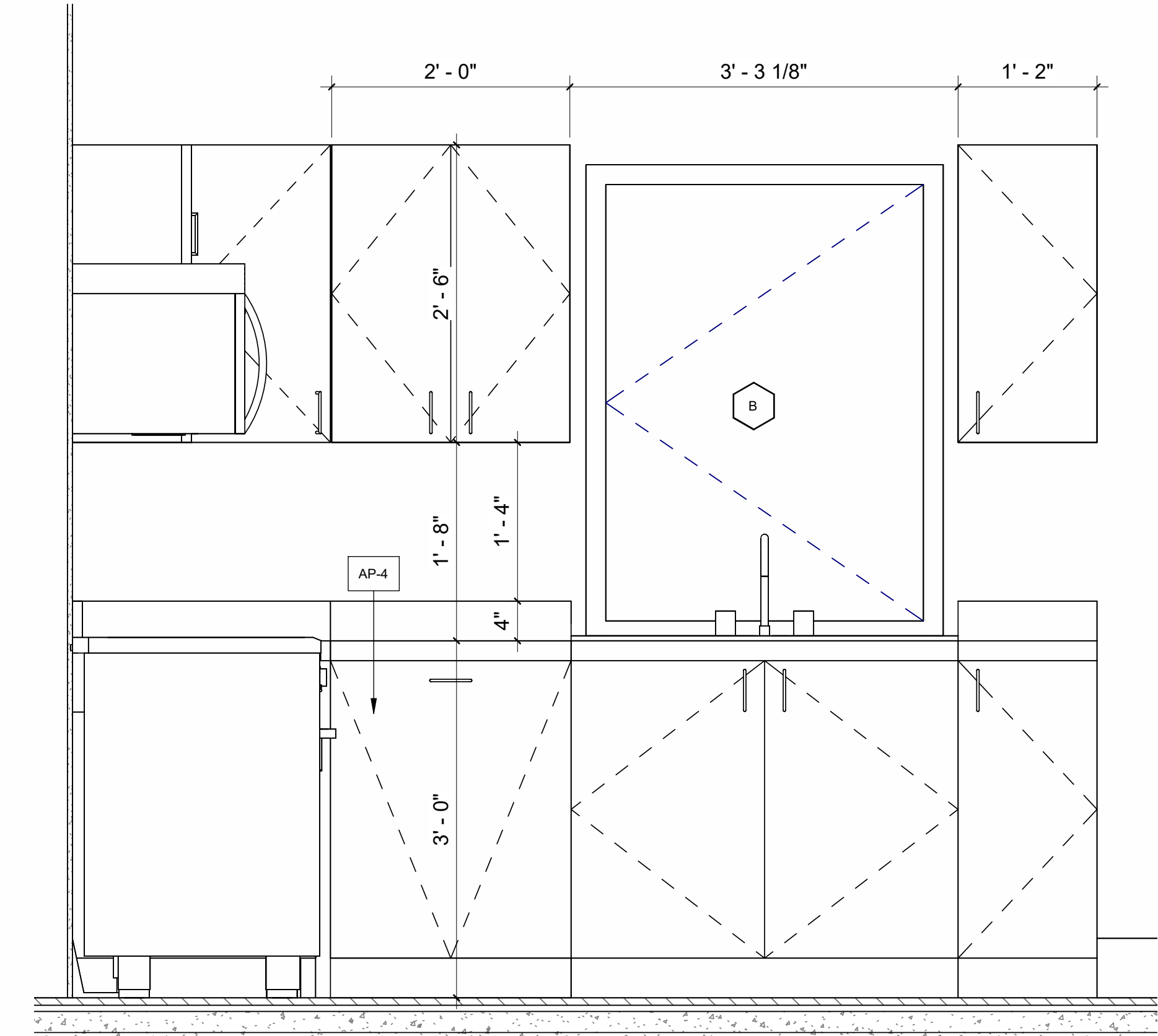
2 MILLWORK VIEW 2 1" = 1'-0"
