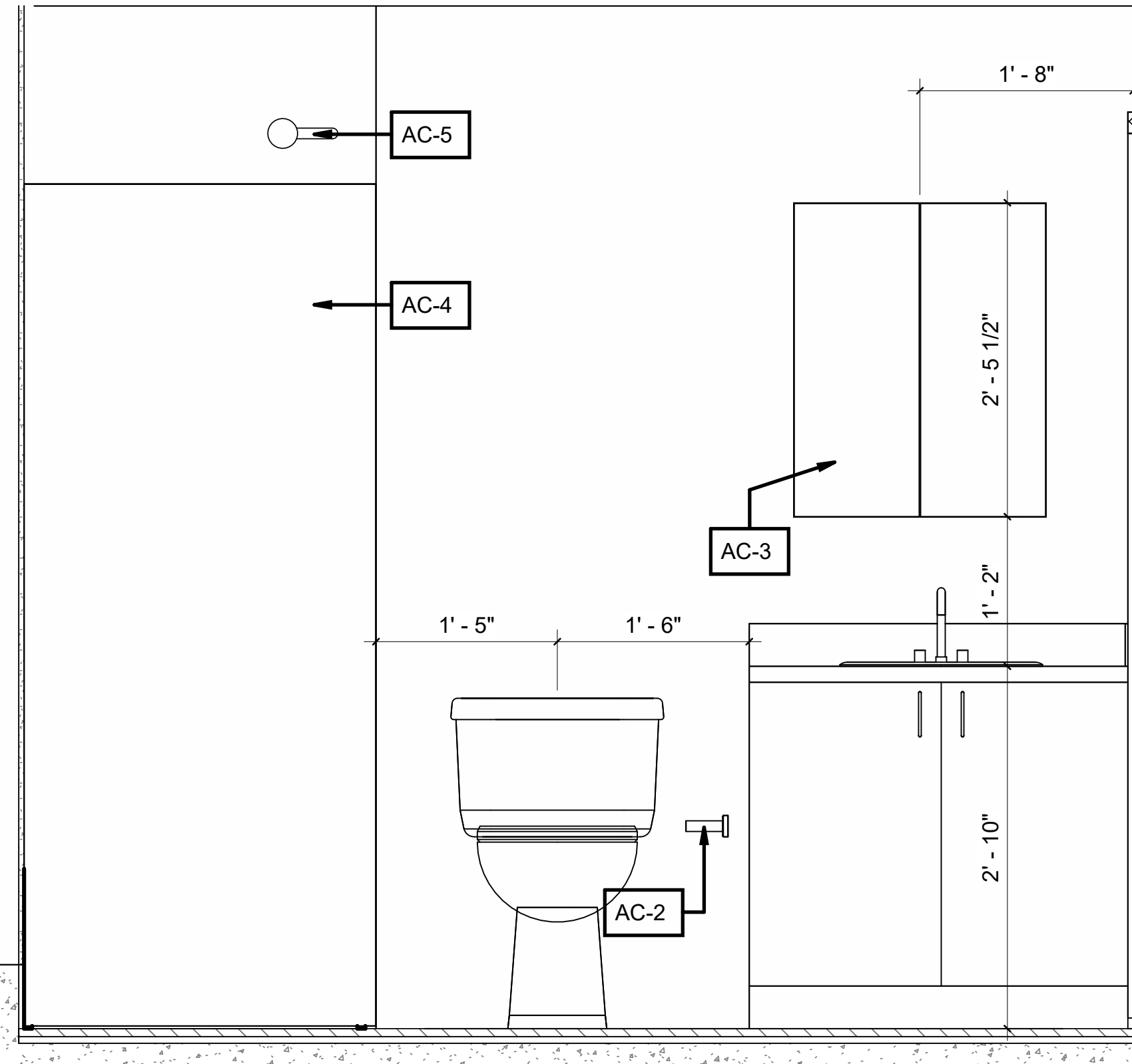
9 Elevation 1 - c A-600 1" = 1'-0"
